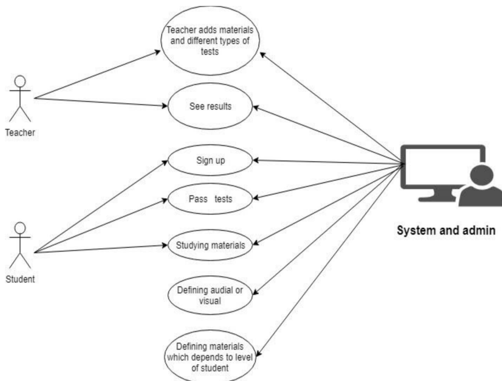
Figure 4.2 – Use-case diagram
