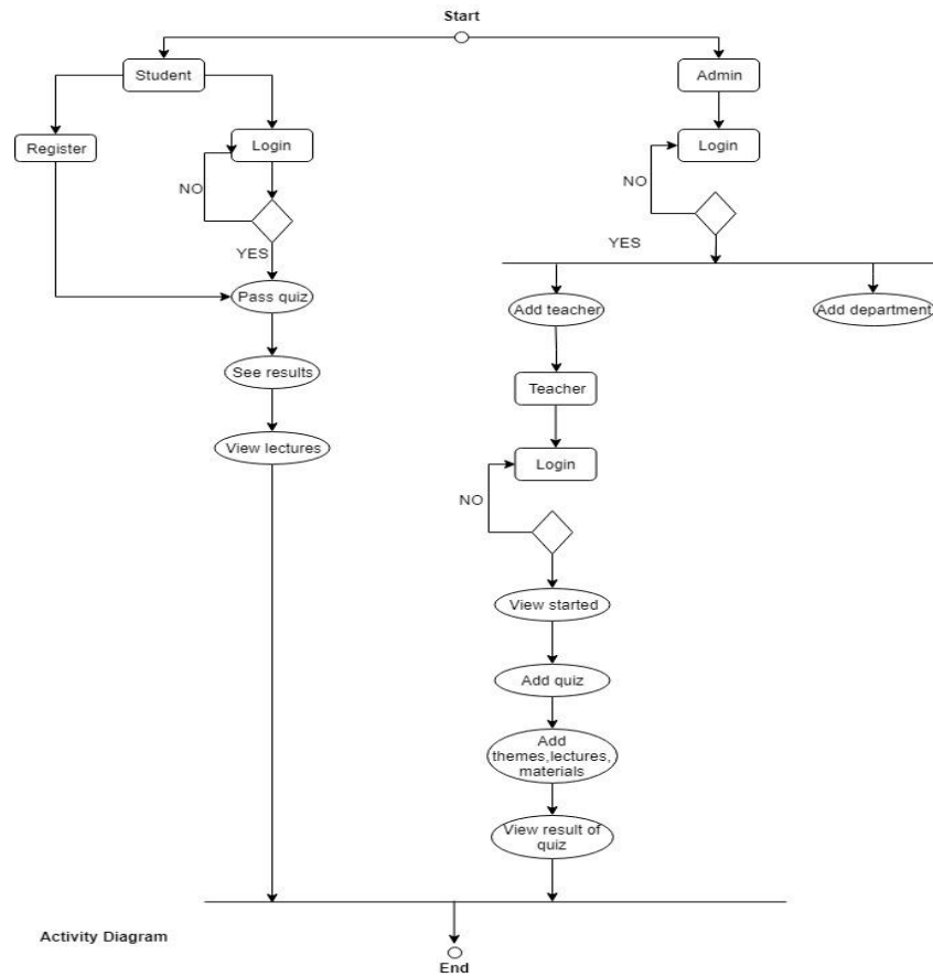
Figure 4.3 – Activity diagram
