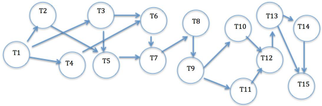
Figure 3.2 – Source infinite graph G_T
